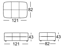
Upholstered bench element
